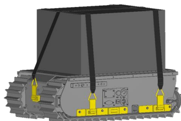
Ensemble attache E-Tracks
